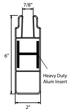
Side view of HD Alum insert
